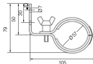
Wandhalterung SL POWER, StreamLED 2 SL50, Art.-Nr. 840082
