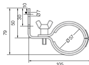
Wandhalterung SL POWER, StreamLED 2 SL50, Art.-Nr. 840082
